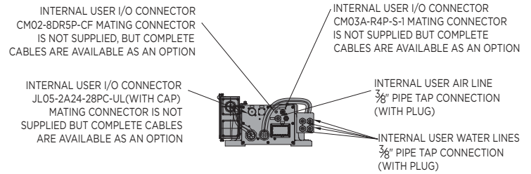
VIEW C
