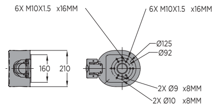
VIEW B
