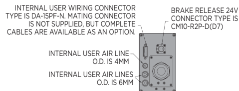
VIEW C
