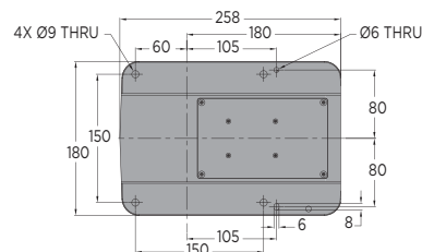
VIEW C
