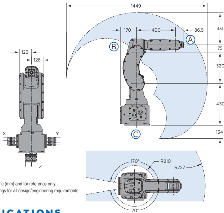
VIEW B
