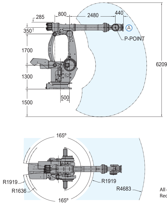
VIEW A
